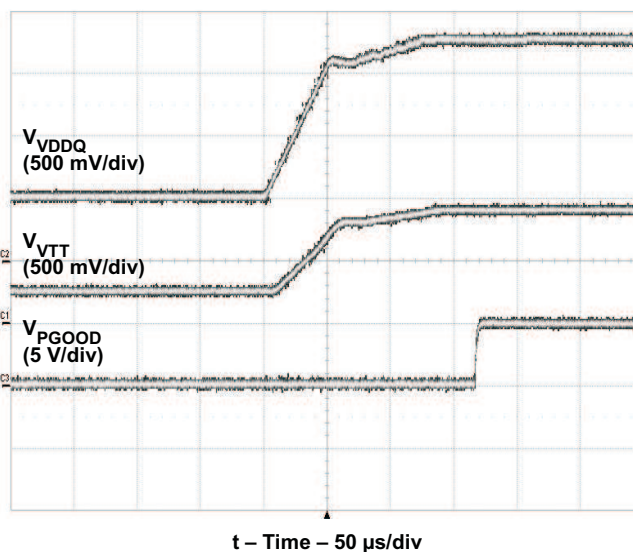
Figure 31. Pre-Biased Start-Up: VDDQ, VTT, and PGOOD
