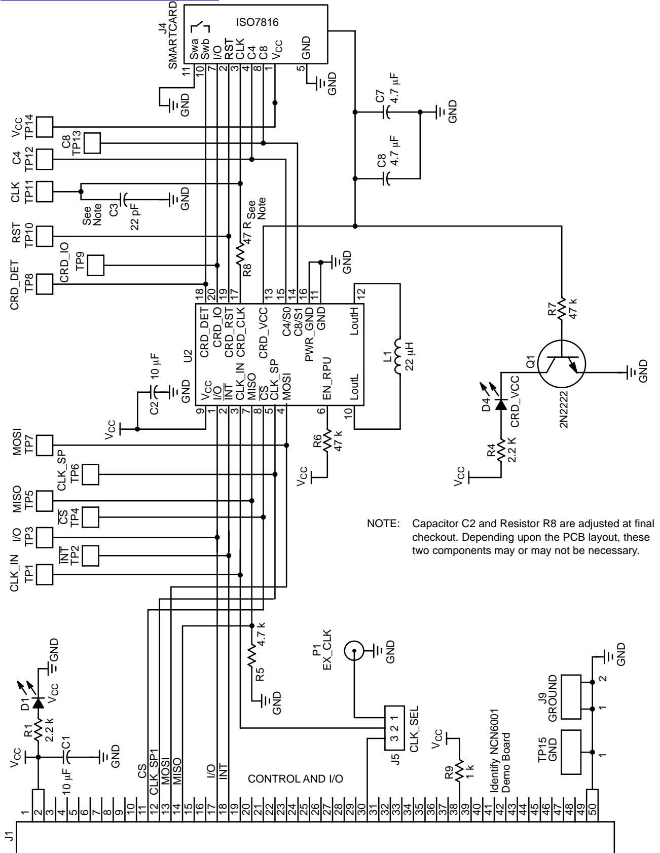
Figure 31. NCN6001 Engineering Test Board Schematic Diagram
