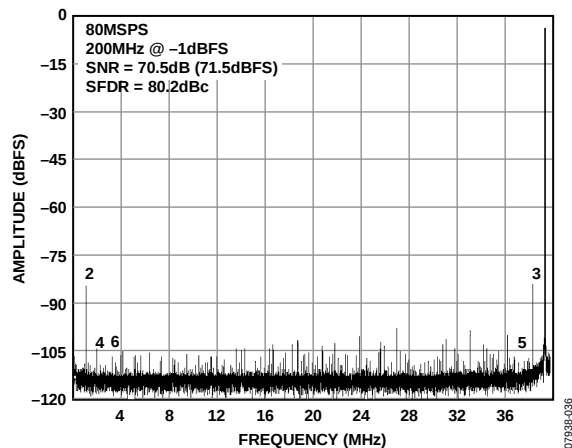
Figure 10. AD9251-80 Single-Tone FFT with f_{IN} = 200 MHz
