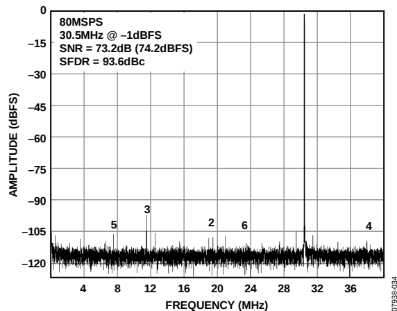
Figure 9. AD9251-80 Single-Tone FFT with f_{IN} = 30.5 MHz
