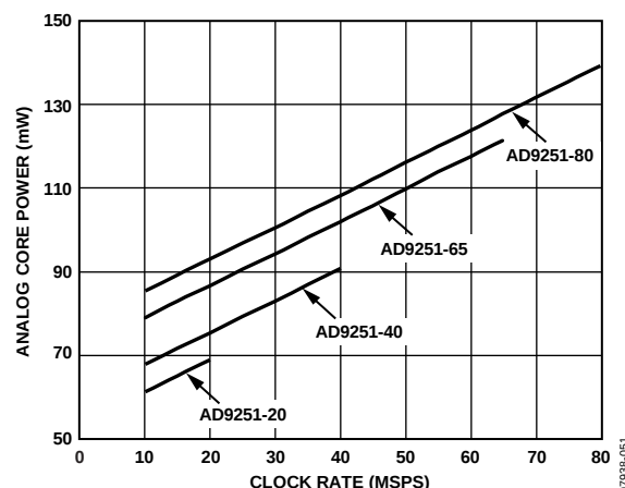
Figure 57. AD9251 Analog Core Power vs. Clock Rate
