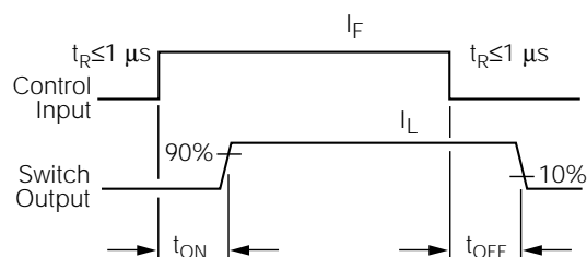
Figure 14. Switching waveform
