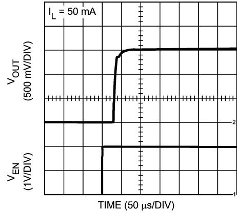
Enable Start Up Timing, ( V_{OUT} = 1.5V )
