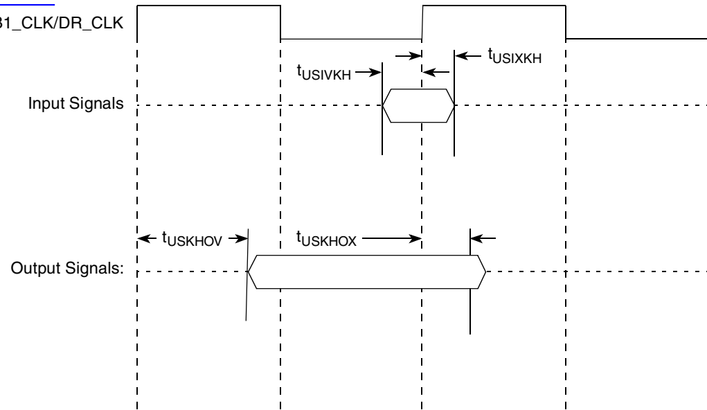
Figure 37. USB Signals
