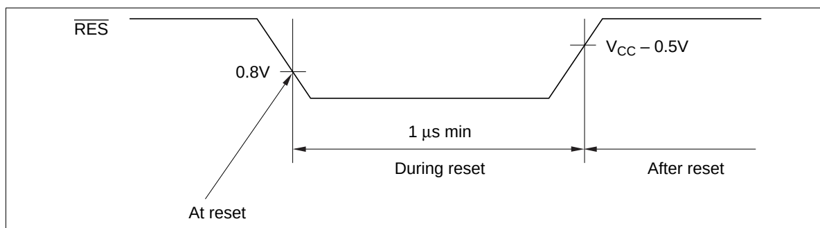
Figure 35 Reset Definition
