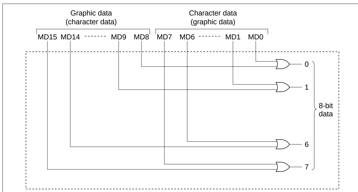
Figure 18 OR Function
