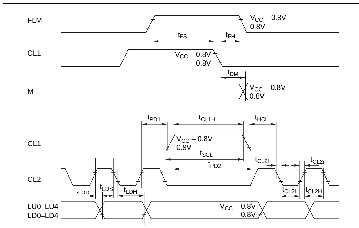
Figure 39 LCD Interface
