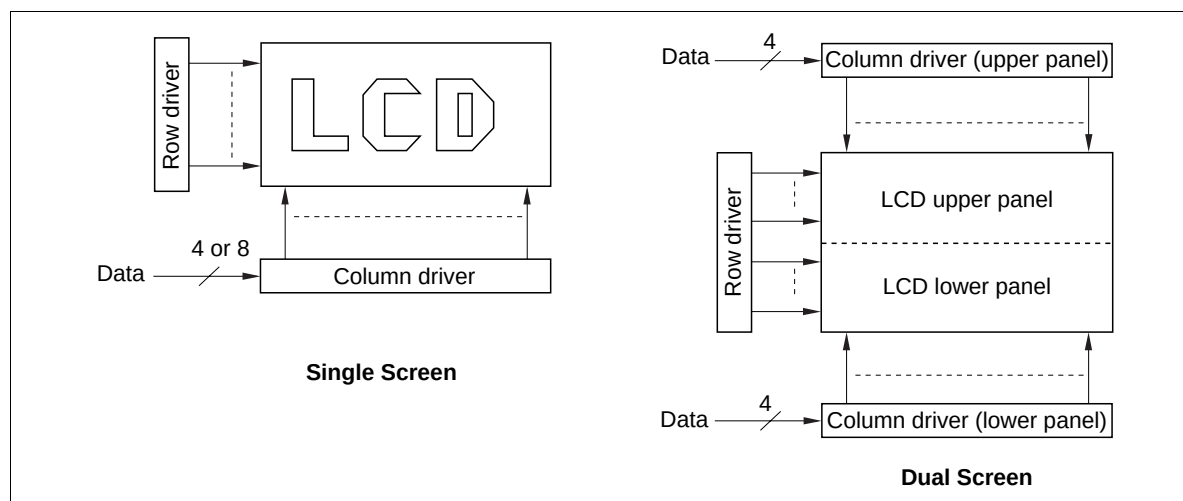
Figure 21 Hardware Configuration According to Screen Format
