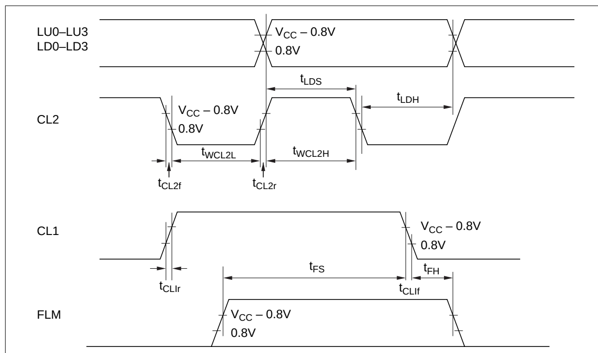
Figure 38 LCD Interface
