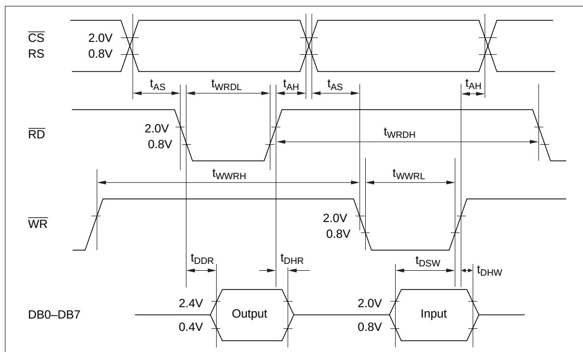
Figure 36 CPU Interface
