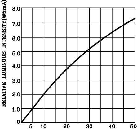
Fig.5 RELATIVE LUMINOUS INTENSITY
