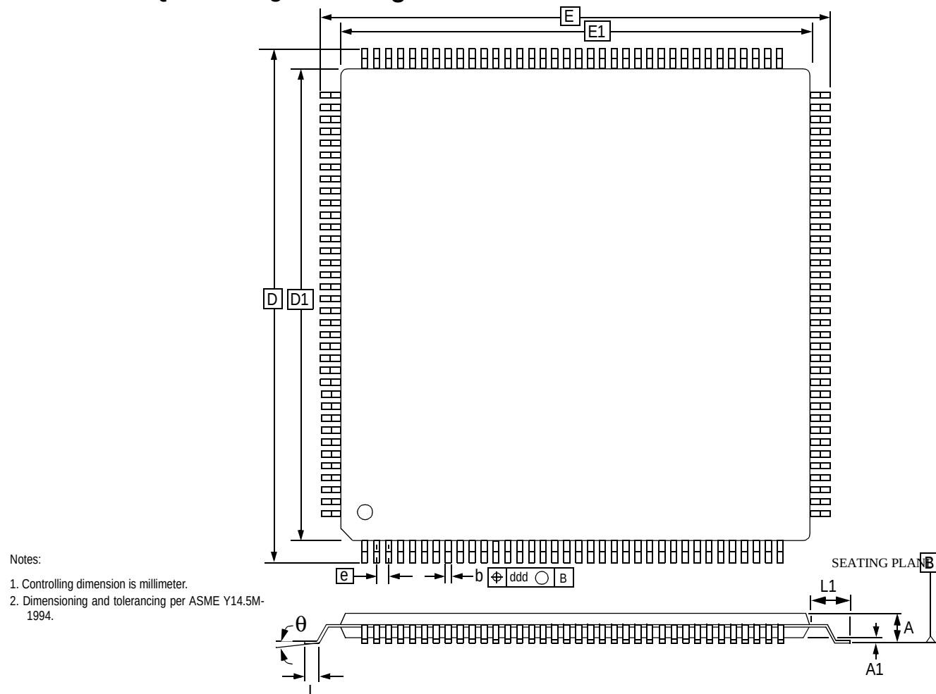
Figure 22. 144-Pin LQFP Package Drawing
