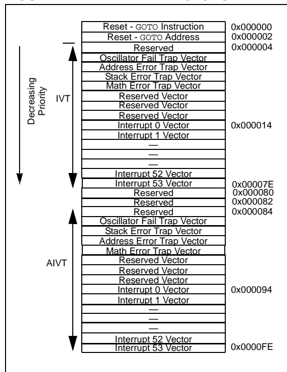
FIGURE 4-1: TRAP VECTORS
