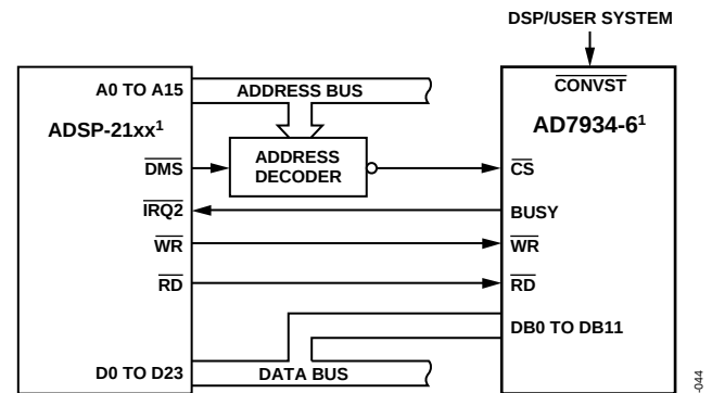
Figure 41. Interfacing to the ADSP-21xx
