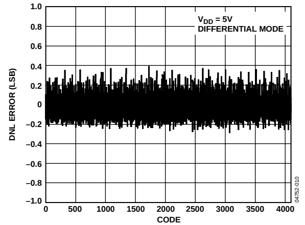
Figure 7. Typical DNL @ V_{DD} = 5\text{V}
