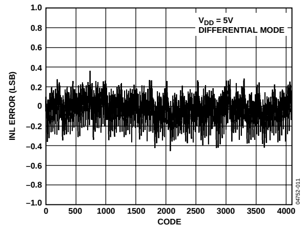
Figure 8. Typical INL @ V_{DD} = 5\text{V}
