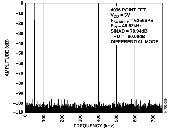
Figure 6. FFT @ V_{DD} = 5\text{V}
