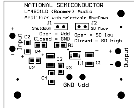
Silk Screen
