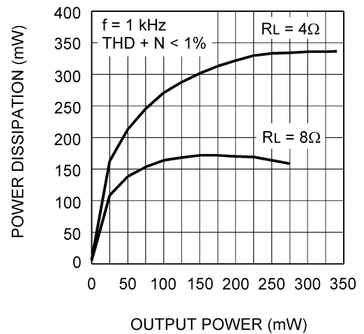
Power Dissipation vs Output Power, V_{DD}=2.6V
