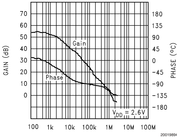
Open Loop Frequency Response, 2.6V
