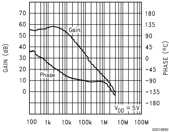
Open Loop Frequency Response, 5V
