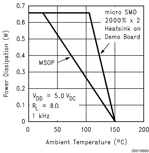
Power Derating Curves
