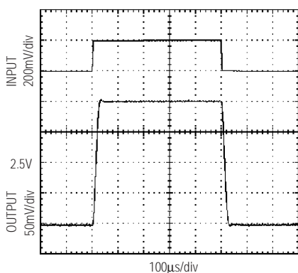
MAX951/MAX953 OP-AMP SMALL-SIGNAL TRANSIENT RESPONSE
