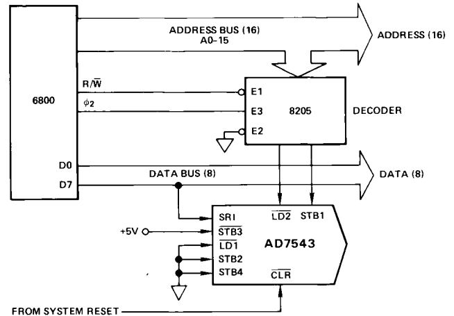
Figure 8. AD7543-MC6800 Interface
