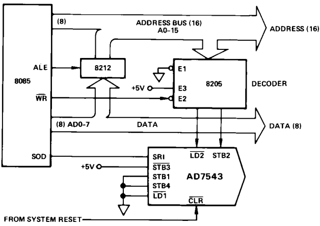
Figure 9. AD7543-8085 Interface
