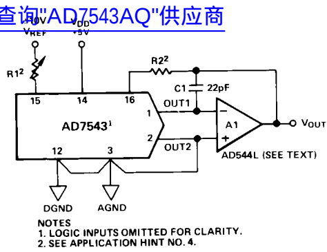
Figure 6. Unipolar Binary Operation (2-Quadrant Multiplication)
