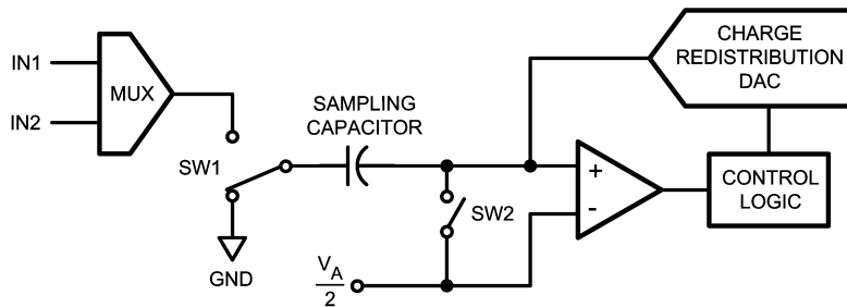
FIGURE 2. ADC122S021 in Hold Mode
