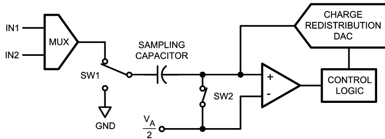
FIGURE 1. ADC122S021 in Track Mode
