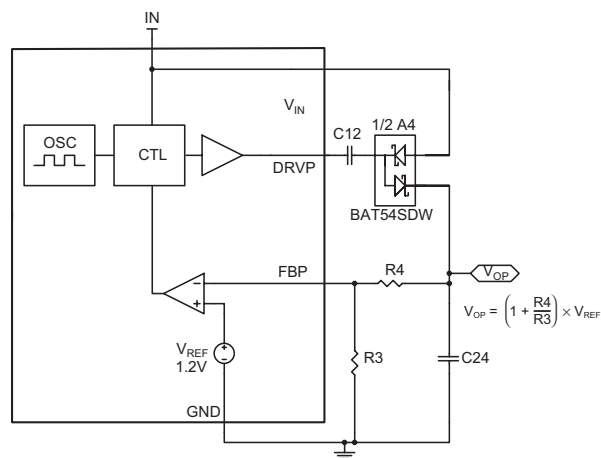
Figure 2: Postive Charge Pump Block Diagram.
