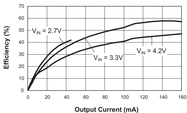
5V Output Efficiency vs. Output Current ( V_{OUT} = 5V ; V_{POS} = 12.5V @ 10mA; V_{NEG} = -7.8V @ 5mA)
