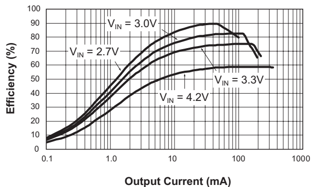
5V Output Efficiency vs. Output Current (No-Load at V_{POS} and V_{NEG} )
