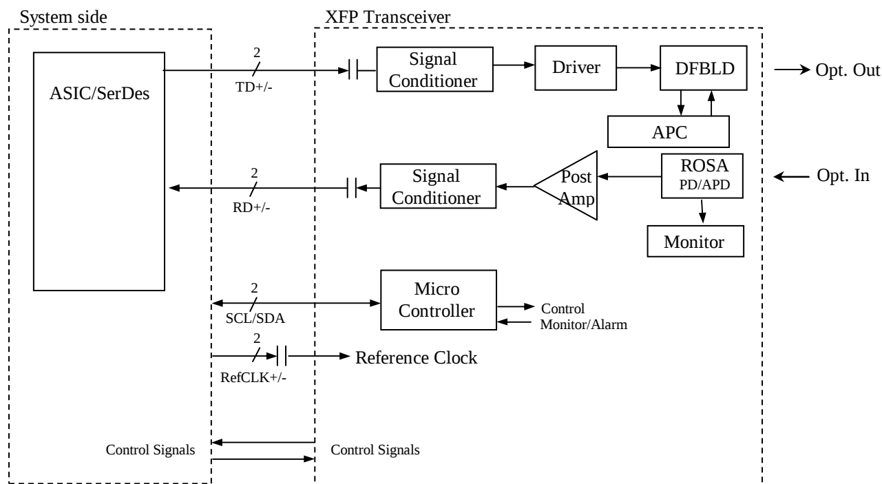
Fig. 2.1 Block Diagram
