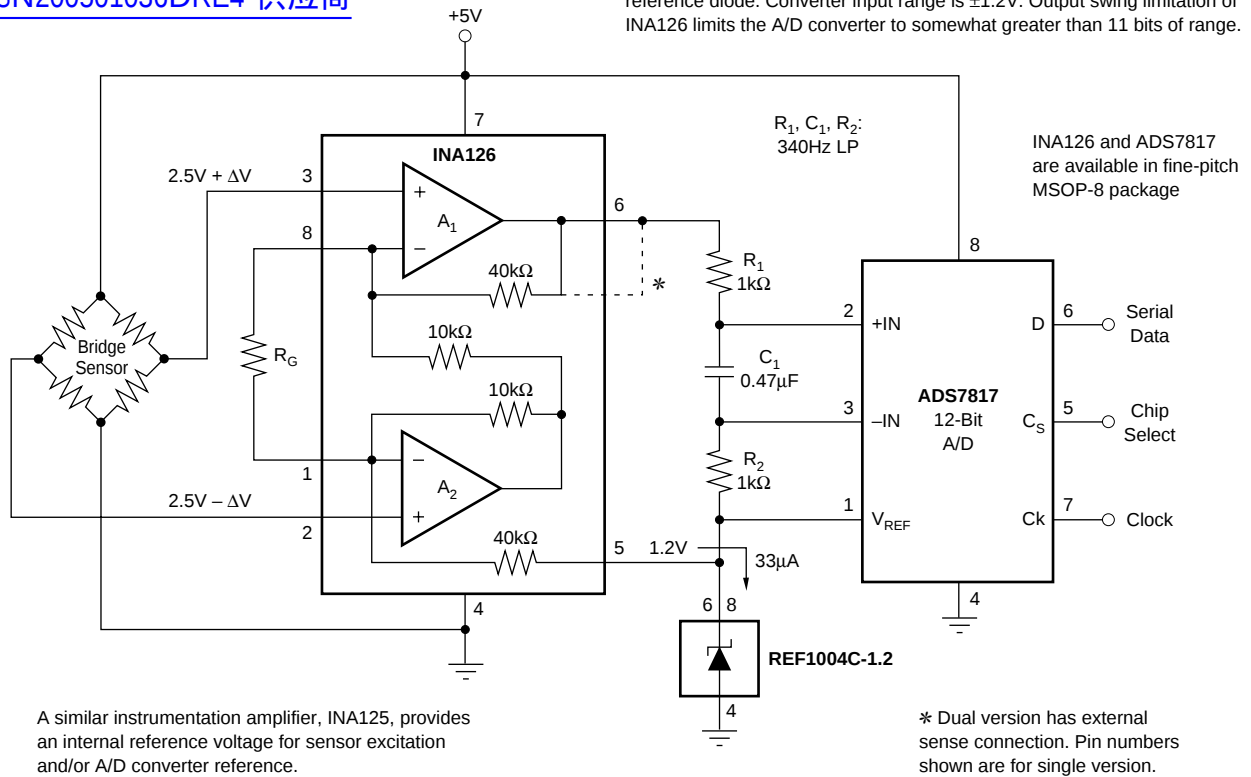
FIGURE 4. Bridge Signal Acquisition—Single 5V Supply.
