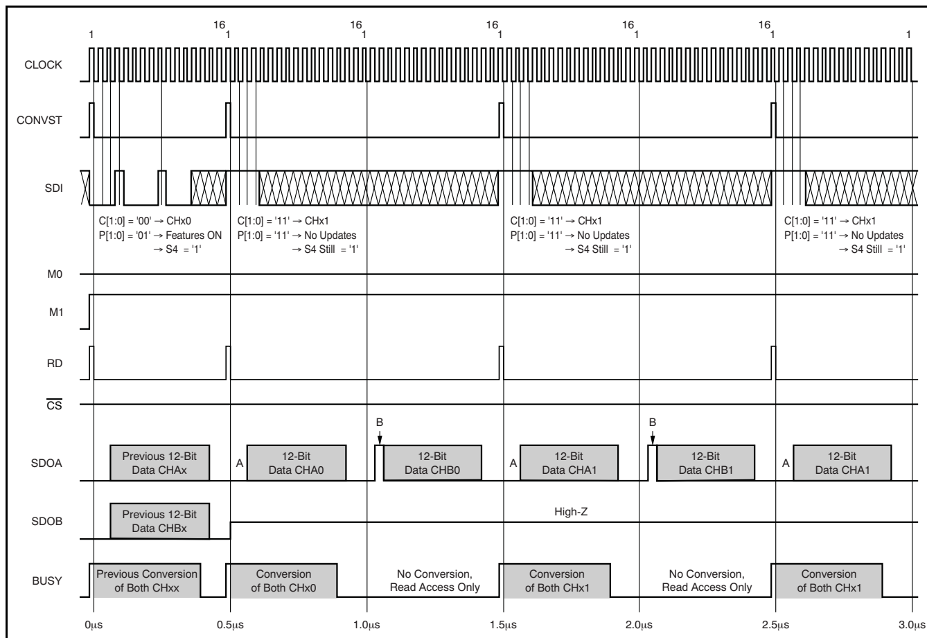
Figure 36. Special Mode II Timing Diagram (M0 = 0; M1 = 1; S4 = 1)
