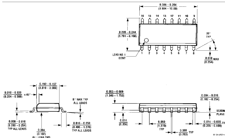
14 Lead Small Outline Integrated Circuit (S) NS Package Number M16A
