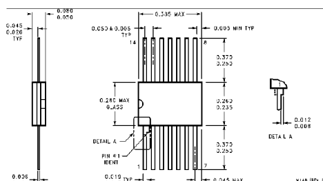
14 Lead Ceramic Flatpak (F) NS Package Number W14B
