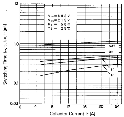
Switching Time
