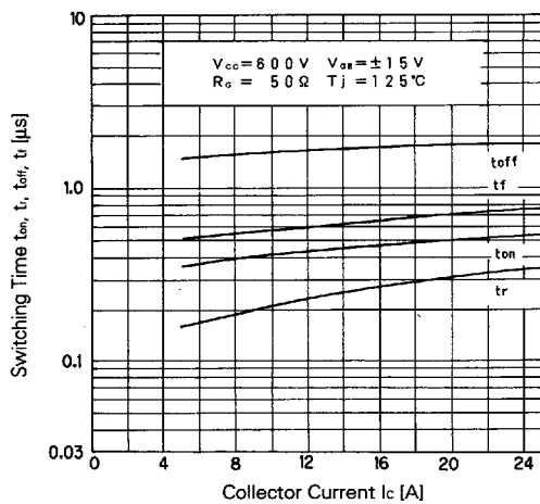
Switching Time
