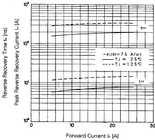
T_{rr}, I_{rr}-I_f
