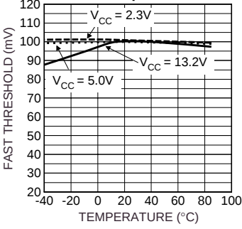
Circuit Breaker Fast ( V_{TRIP} ) vs. Temperature
