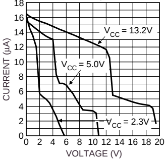
Gate Current vs. Gate Voltage @ 25°C
