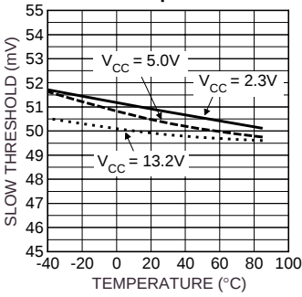
Circuit Breaker Slow ( V_{TRIP} ) vs. Temperature
