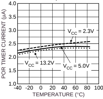
Power-On Reset Timer Current vs. Temperature
