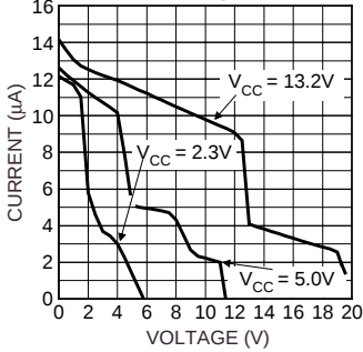
Gate Current vs. Gate Voltage @ 85°C
