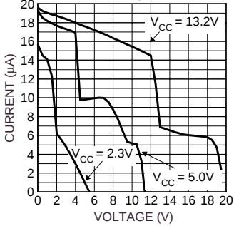
Gate Current vs. Gate Voltage @ -40°C
