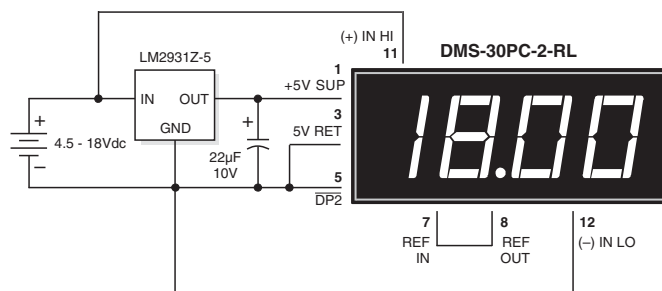
Figure 8. 4.5-18V Power Supply Monitor
