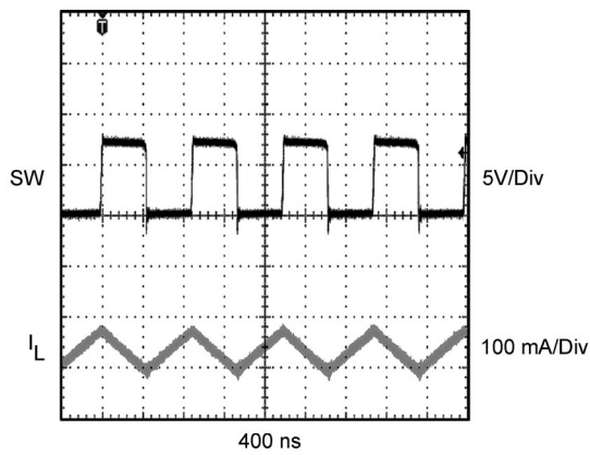
V_{IN} = 3.6V at 15mA & 2 Leds
