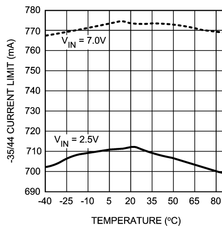
Current Limit (LM3503-35/44) vs Temperature
