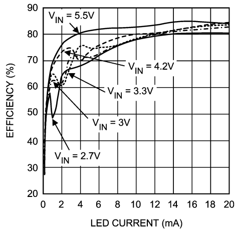
6 LED Efficiency vs LED Current
