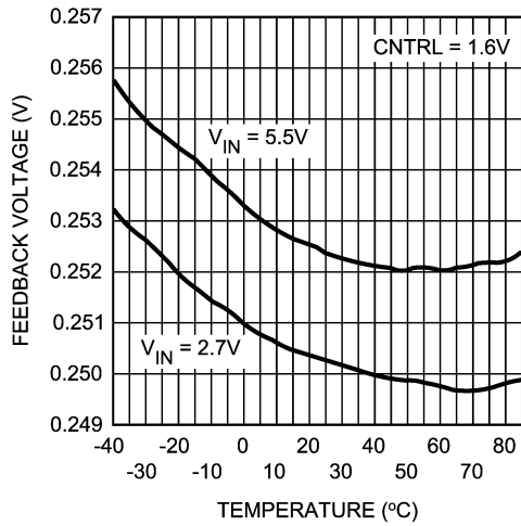
Feedback Voltage ( V_{Cntrl} = 1.6V ) vs Temp
