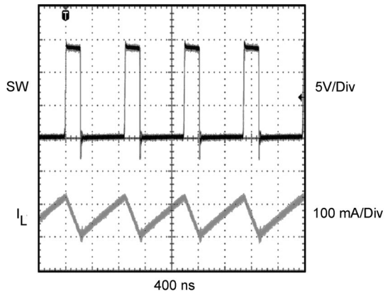
V_{IN} = 3.6V at 15mA & 4 Leds
