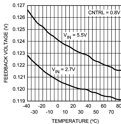
Feedback Voltage ( V_{CNTRL} = 0.8V ) vs Temp
