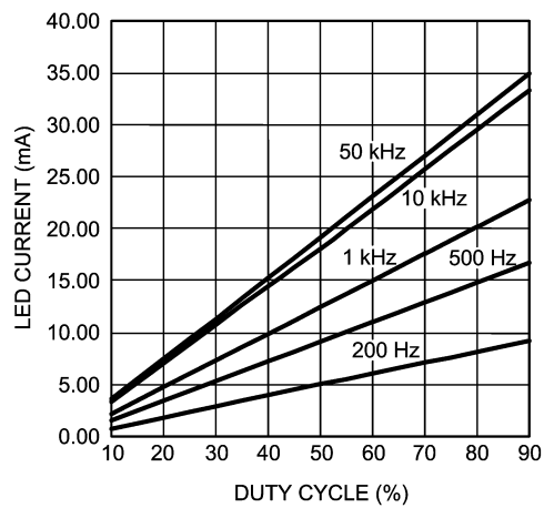
Dimming Duty Cycle vs. LED Current V_{IN} = 3.6V , 2LEDs on Main & Sub Display
