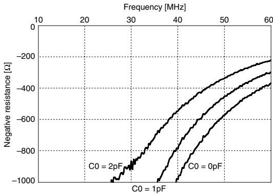
5027x1 to x7, V_{DD} = 3.3\text{V} , T_a = 25^\circ\text{C}
