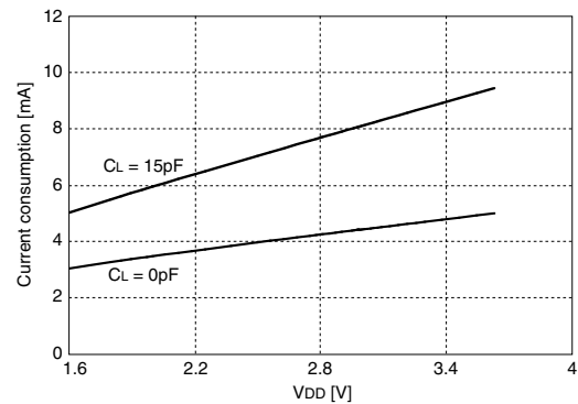
5027xD, f OUT = 85MHz, Ta = 25°C
