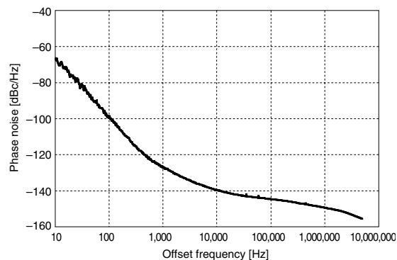
5027AP, V_{DD} = 3.3\text{V} , f_{OSC} = f_{OUT} = 80\text{MHz} , T_a = 25^\circ\text{C}
