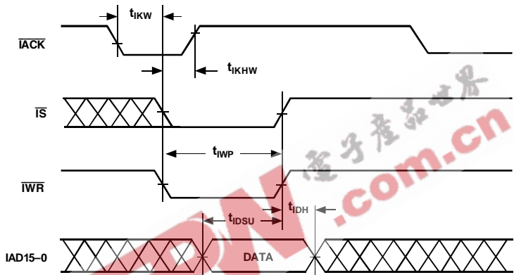
Figure 31. IDMA Write, Short Write Cycle
