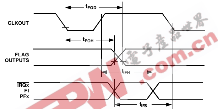
Figure 25. Interrupts and Flags
