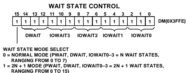
Figure 9. Wait State Control Register
