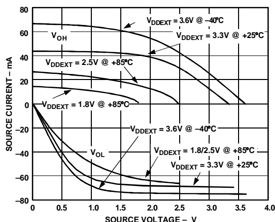
Figure 19. Typical Output Driver Characteristics for V_{DDEXT} at 3.6 V, 3.3 V, 2.5 V, and 1.8 V
