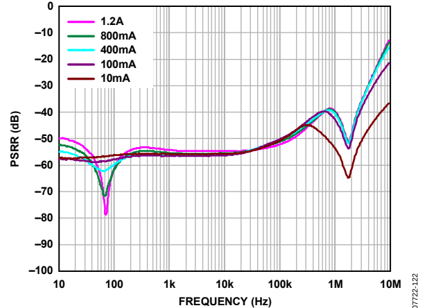
Figure 22. Power Supply Rejection Ratio vs. Frequency, V_{OUT} = 2.5\text{ V} , V_{IN} = 3.5\text{ V}
