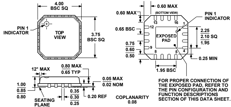
Figure 49. 16-Lead Lead Frame Chip Scale Package [LFCSP_VQ] 4 mm × 4 mm Body, Very Thin Quad (CP-16-4) Dimensions shown in millimeters
