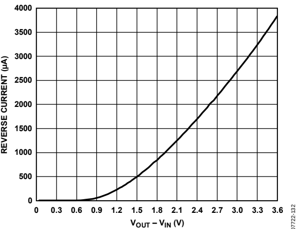
Figure 32. Reverse Current vs. V_{OUT} - V_{IN}
