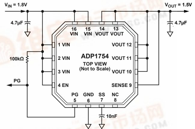
Figure 1. ADP1754 with Fixed Output Voltage, 1.5 V
