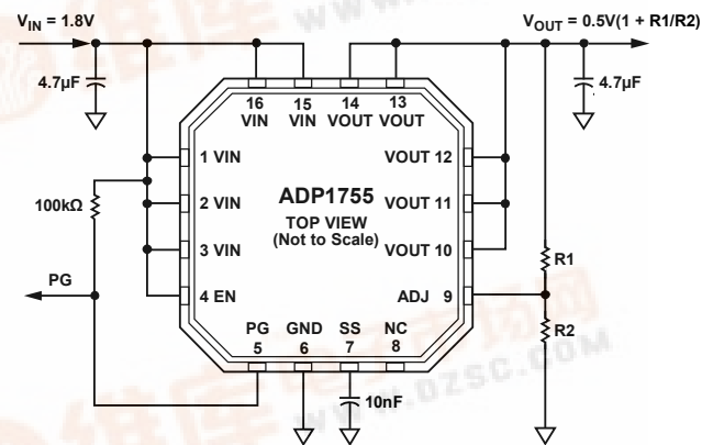
Figure 2. ADP1755 with Adjustable Output Voltage, 0.75 V to 3.0 V
