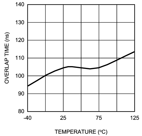
Overlap Time vs Temperature R_{SET} = 38k\Omega
