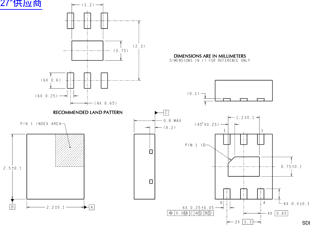
6 Pin LLP NS Package Number SDB06A
