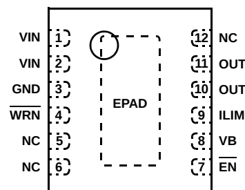
ISL9209B (12 LD 4x3 TDFN) TOP VIEW
