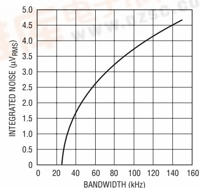
Line Receiver Integrated Noise 25kHz to 150kHz
