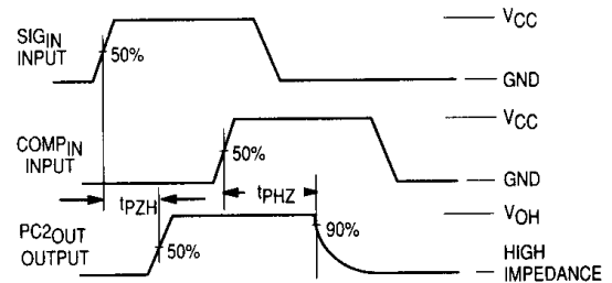
Figure 2. Switching Waveforms
