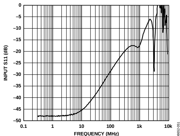
Figure 45. ADV3221/ADV3222 S11 (Including Evaluation Board)
