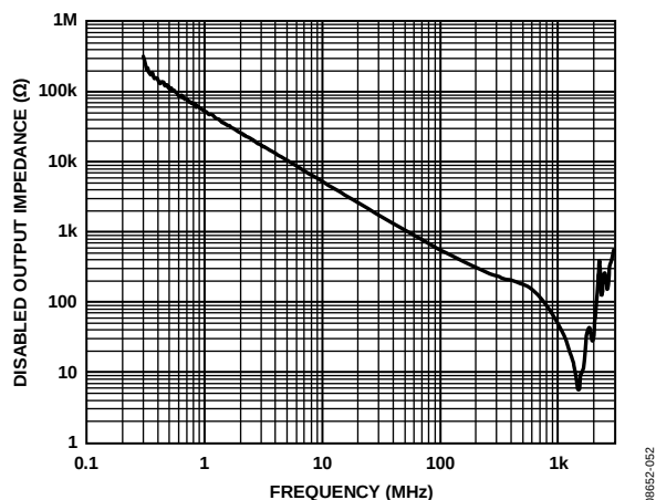
Figure 46. ADV3222 Disabled Output Impedance
