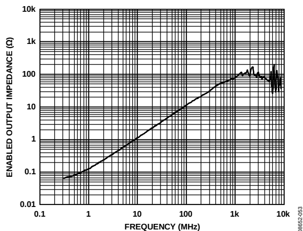
Figure 47. ADV3222 Enabled Output Impedance
