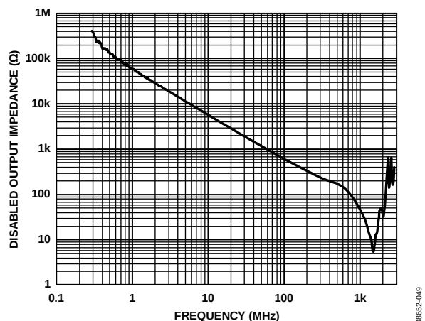
Figure 43. ADV3221 Disabled Output Impedance
