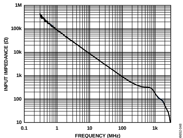
Figure 42. ADV3221/ADV3222 Input Impedance
