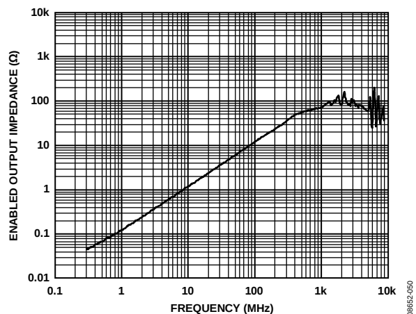
Figure 44. ADV3221 Enabled Output Impedance
