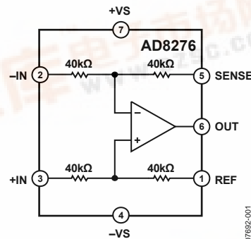
Figure 1. AD8276
