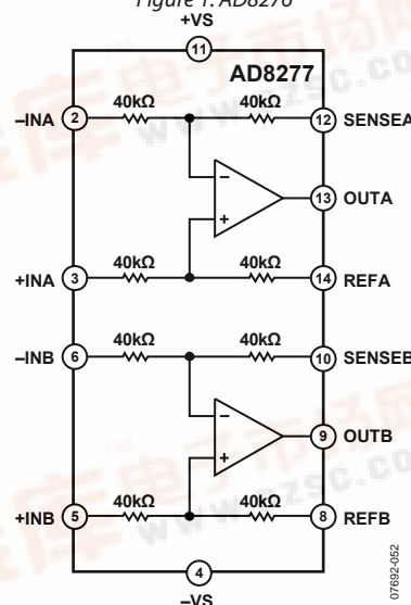
Figure 2. AD8277
