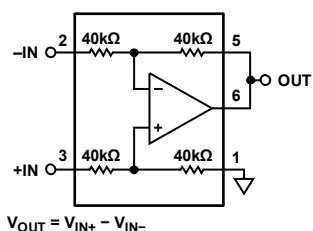
Figure 42. Difference Amplifier, Gain = 1
