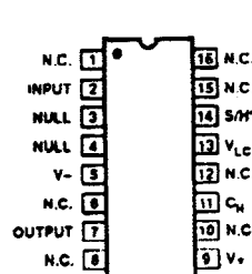
16-PIN SOL (S-Suffix)
