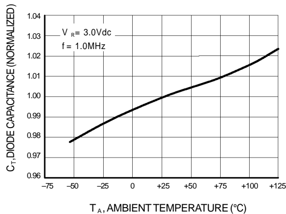
Figure 3. Diode Capacitance
