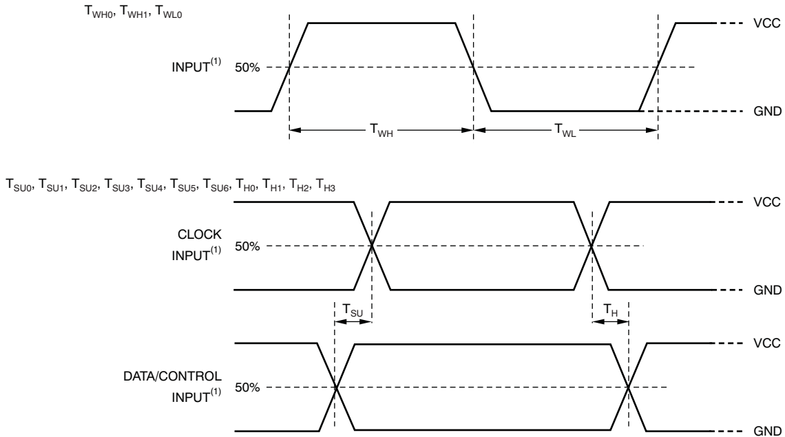
Figure 9. Input Timing
