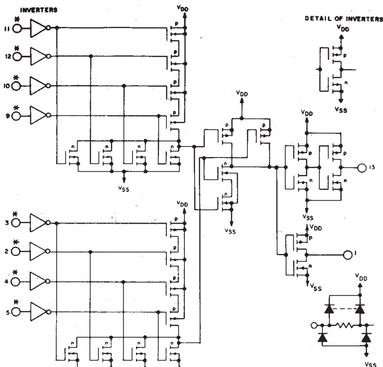
Fig. 7 - Schematic diagram.
