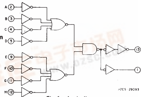
Fig. 1 – Logic diagram.
