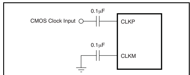
Figure 106. Single-Ended Clock Driving Circuit When DIFF_CLK = 1
