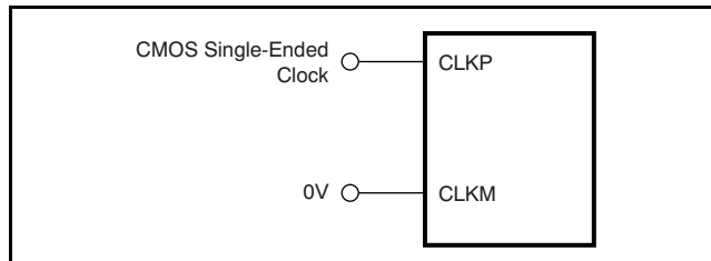
Figure 103. Single-Ended Clock Driving Circuit (DIFF_CLK = 0)
