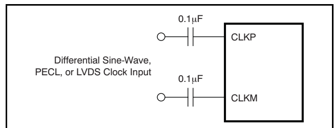
Figure 105. Differential Clock Driving Circuit (DIFF_CLK = 1)
