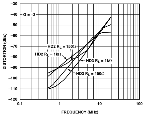
Figure 16. Harmonic Distortion vs. Frequency for Various Loads (See Figure 43)
