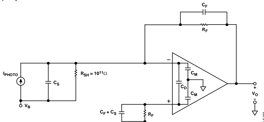
Figure 58. Wideband Photodiode Preamp
