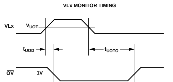
Figure 21. VHx Positive Voltage Monitoring Timing Diagram
