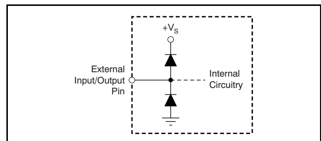
Figure 115. Internal ESD Protection
