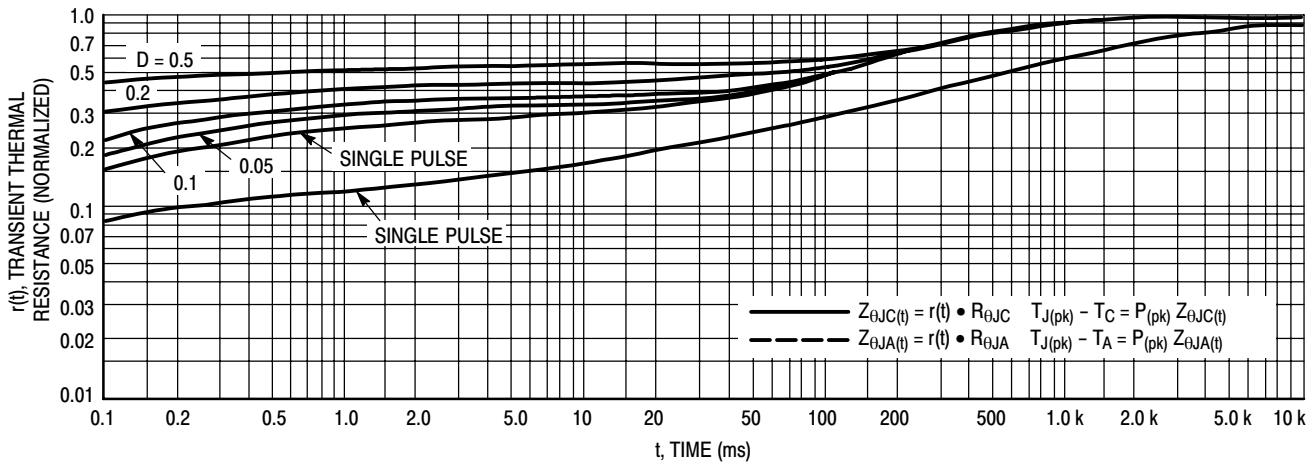
Figure 2. Thermal Response
