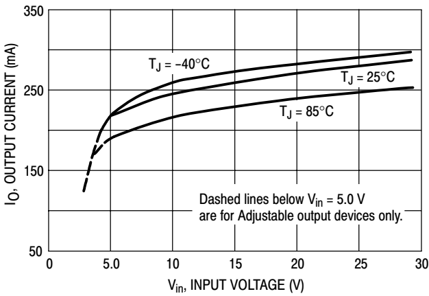
Figure 3. Peak Output Current versus Input Voltage
