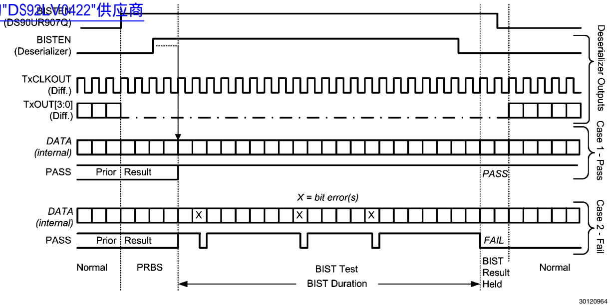
FIGURE 26. BIST Waveforms
