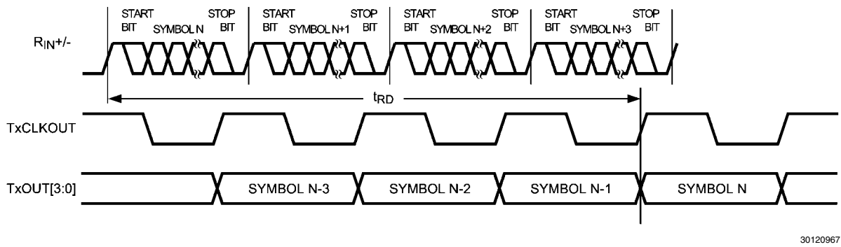
FIGURE 11. DS92LV0422 Latency Delay
