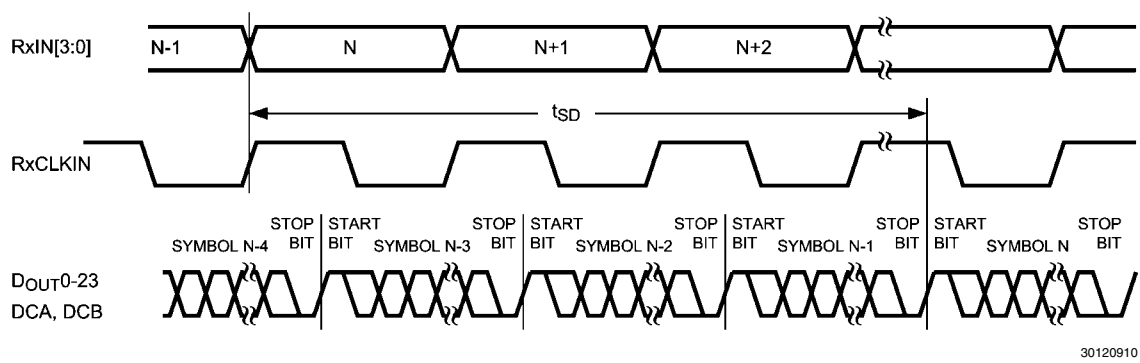
FIGURE 10. DS92LV0421 Latency Delay
