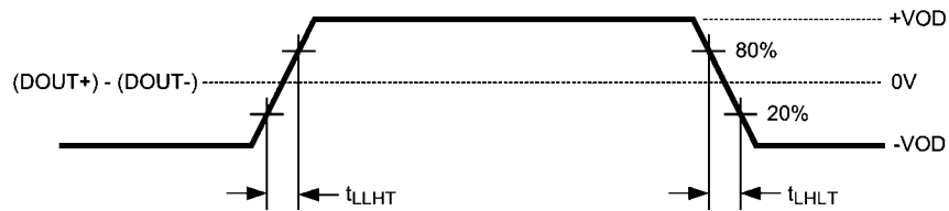
FIGURE 4. Output Transition Times
