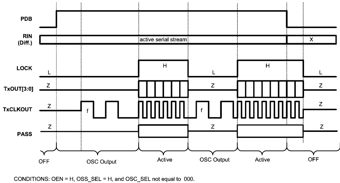
FIGURE 13. DS92LV0422 Output State Diagram
