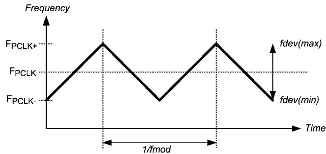
FIGURE 24. SSCG Waveform
