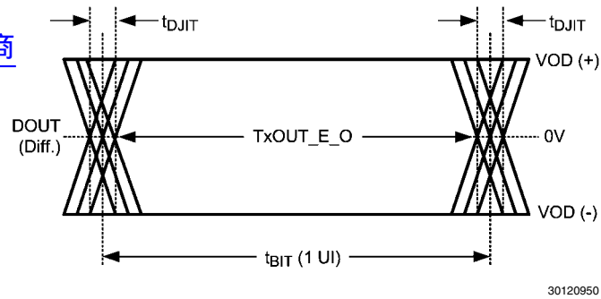
FIGURE 12. DS92LV0421 Output Jitter
