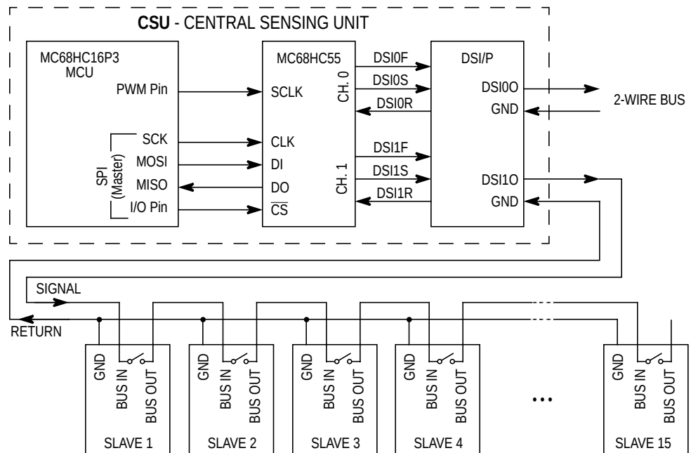
Figure 1-1. DSI System Connections (Other Arrangements Possible)
