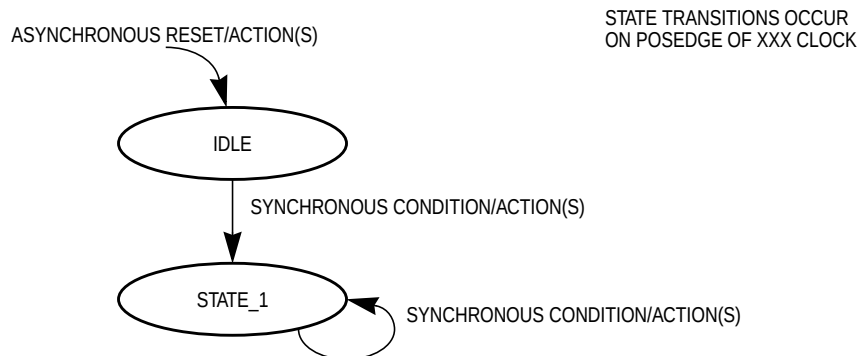
Figure 4-2. State Diagram Notation
