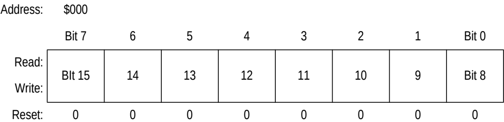
Figure 3-1. DSI Channel 0 Data Register Upper Byte (DSI0H)
