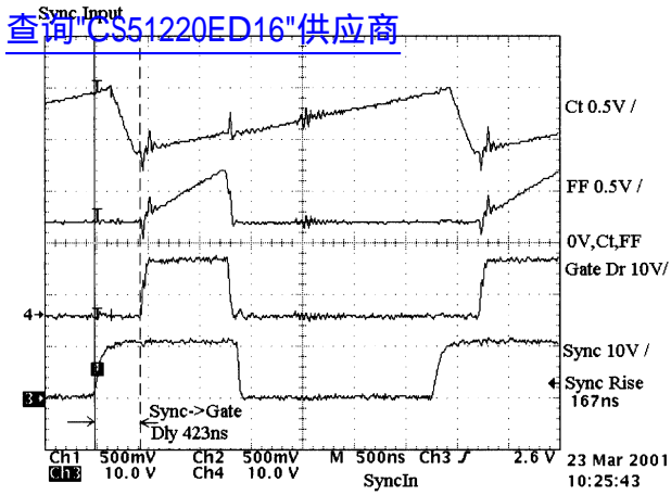
Figure 12. Synchronization Input Timing
