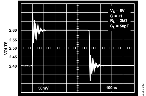
Figure 43. AD8051/AD8052 200 mV Step Response; C_L = 50 pF
