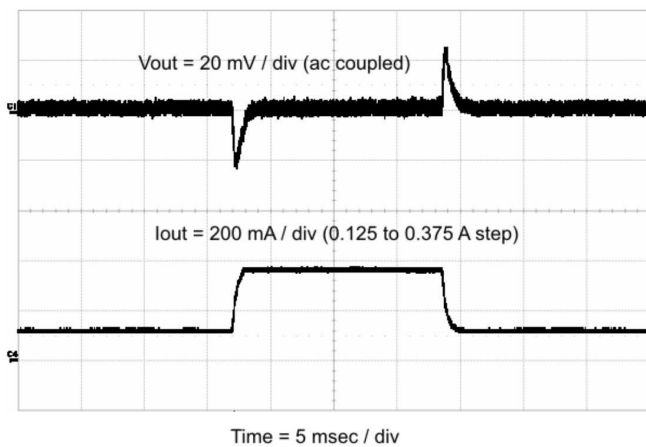
Figure 51. Load Transient
