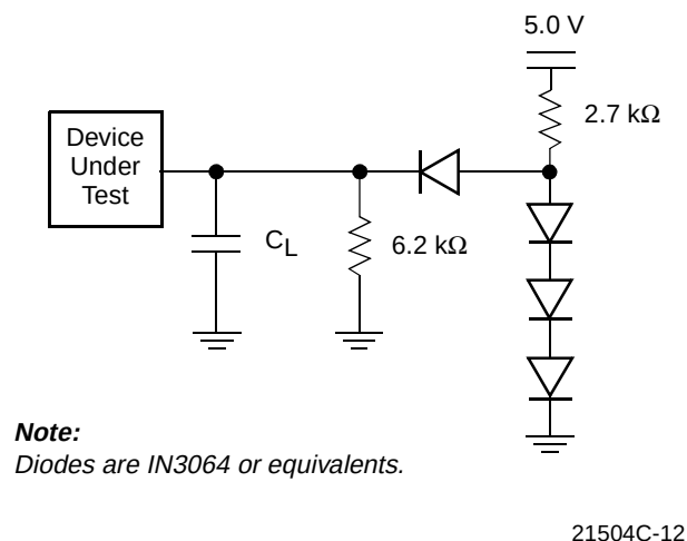
Figure 8. Test Setup
